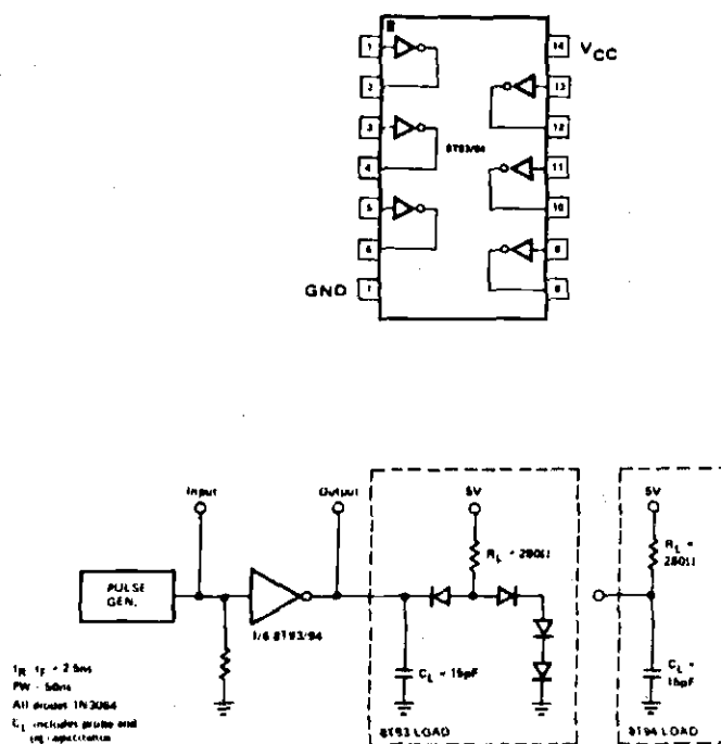
Figure 4-57. High Speed Hex Inverter Connections
