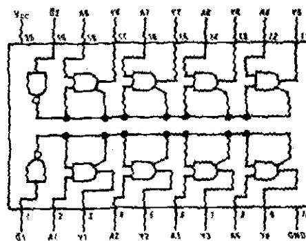
Logic Diagram
