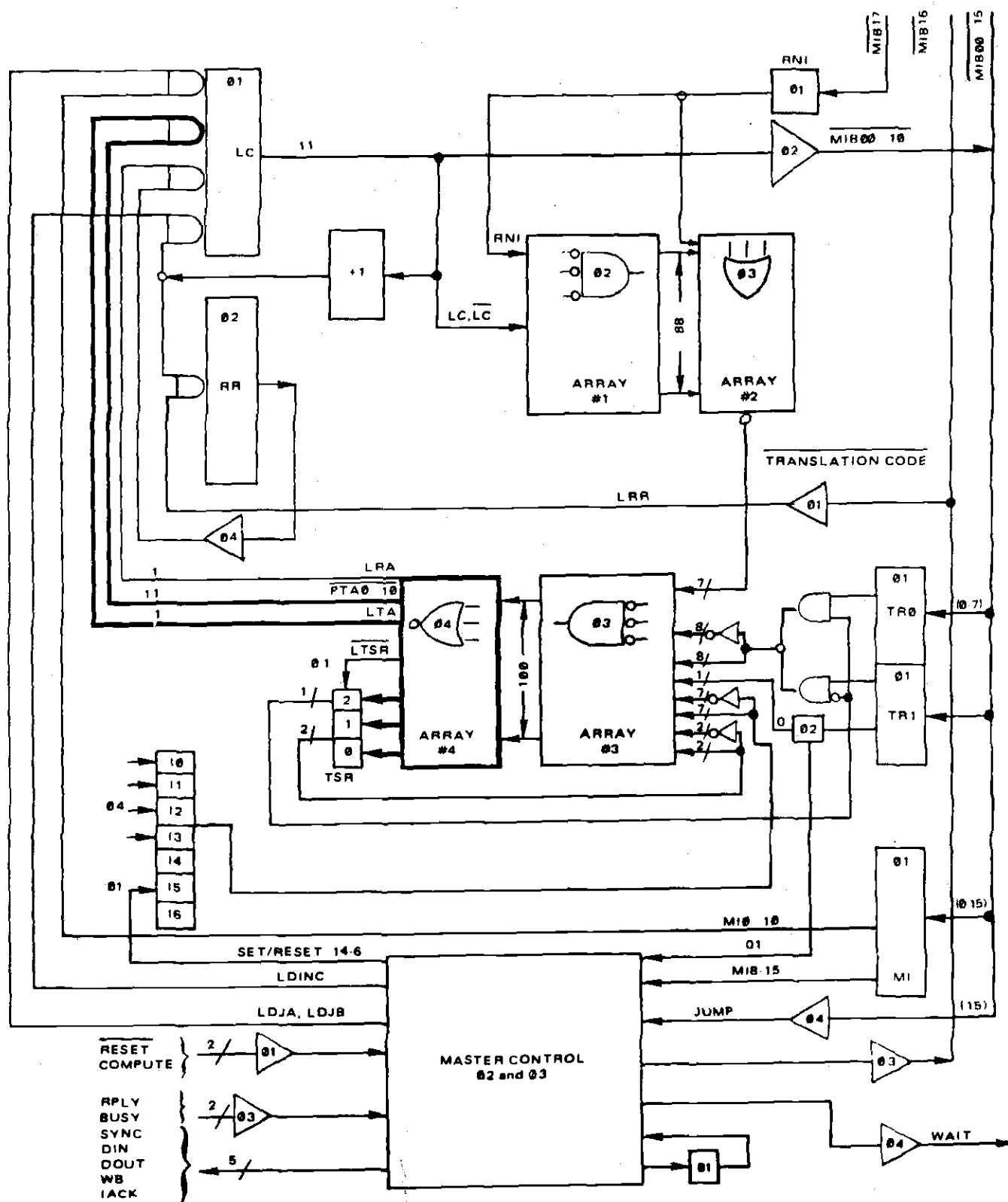
Figure 4-40. 04 Data Flow
