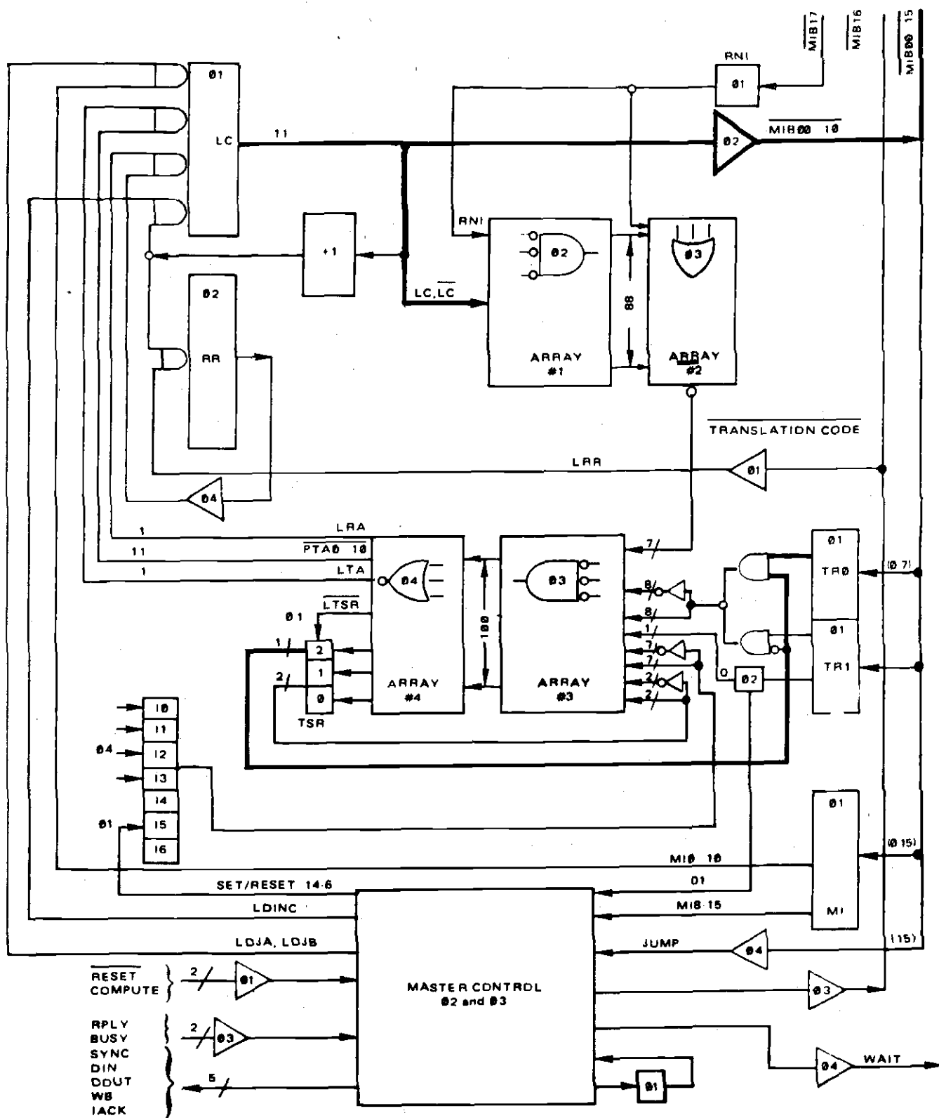
Figure 4-38. 02 Data Flow
