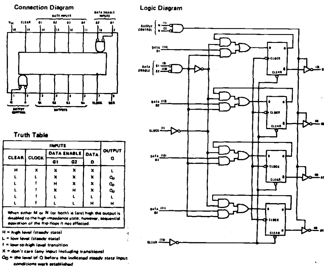
Figure 4-56. Tri-State 4-Bit D Type Register Connections
