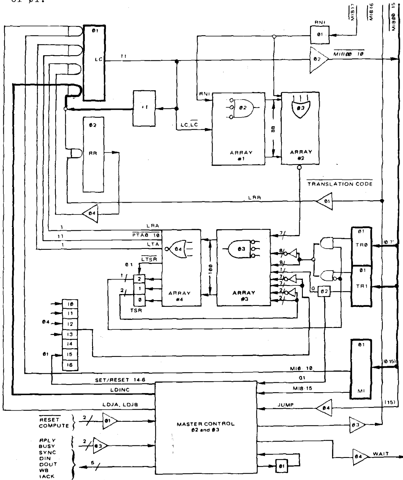
Figure 4-37. 01 Data Flow
