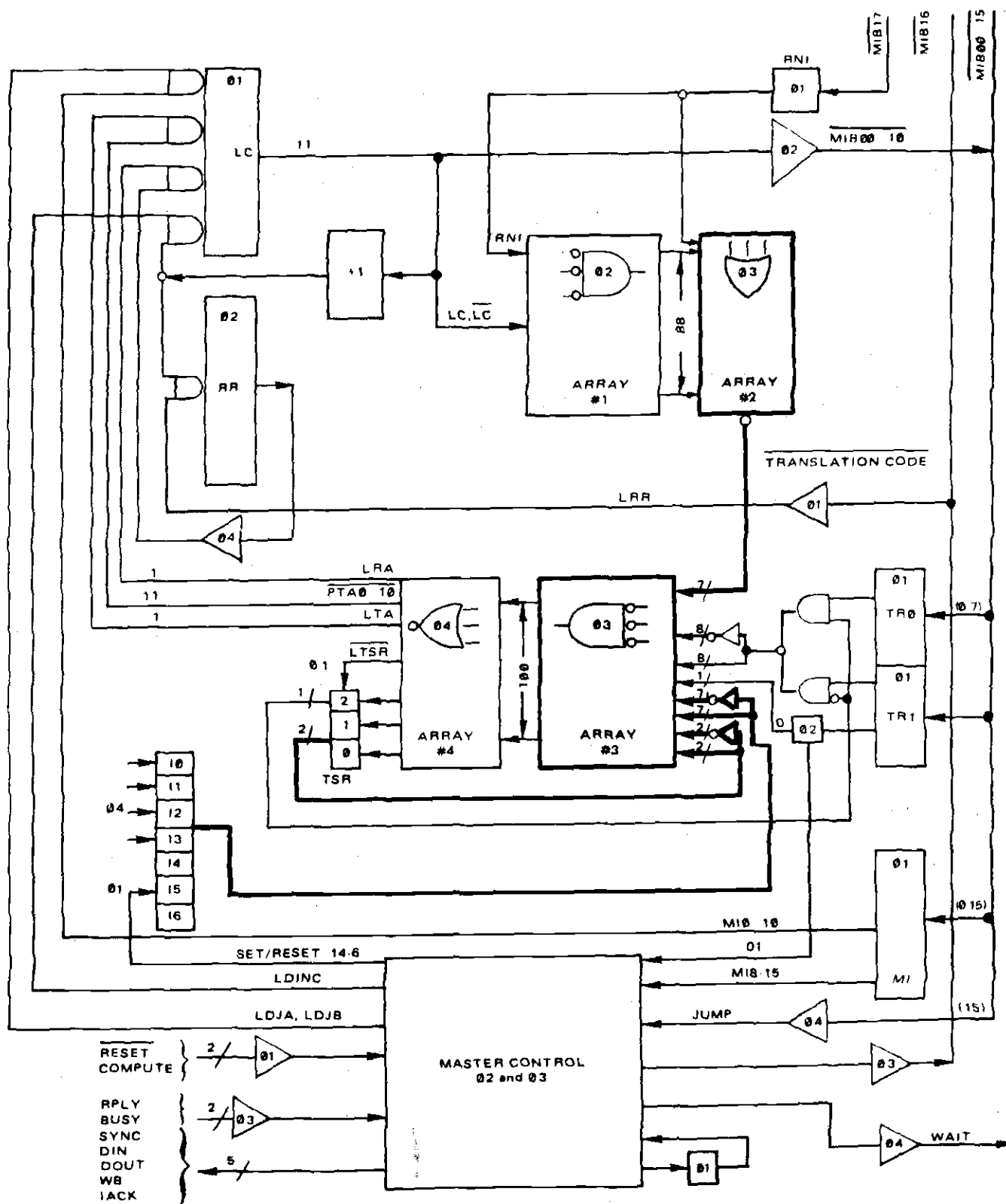
Figure 4-39. 03 Data Flow
