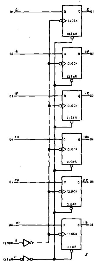
Logic Diagram
