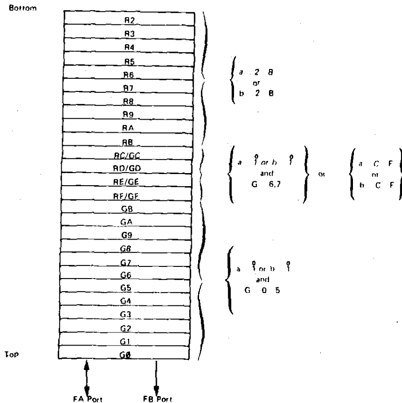
Figure 4-19. Register File
