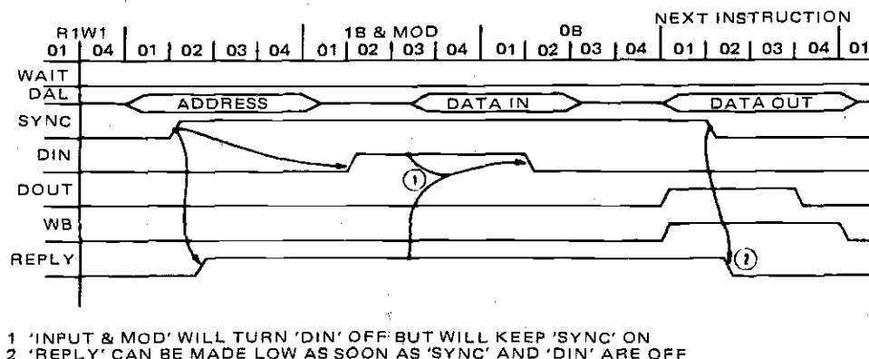
Figure 4-53. Read/Modify/Write Sequence
