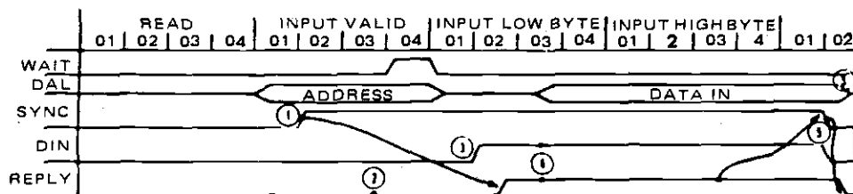
Figure 4-51. Write/Output Sequence
