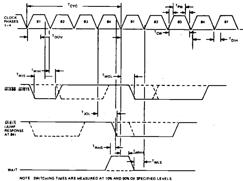
Figure 4-43. Microinstruction Bus Interface Timing
